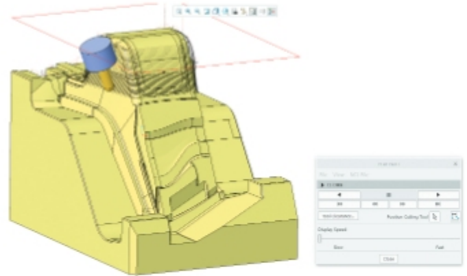
High-speed milling roughing sequence, multi-threaded for fast computation
